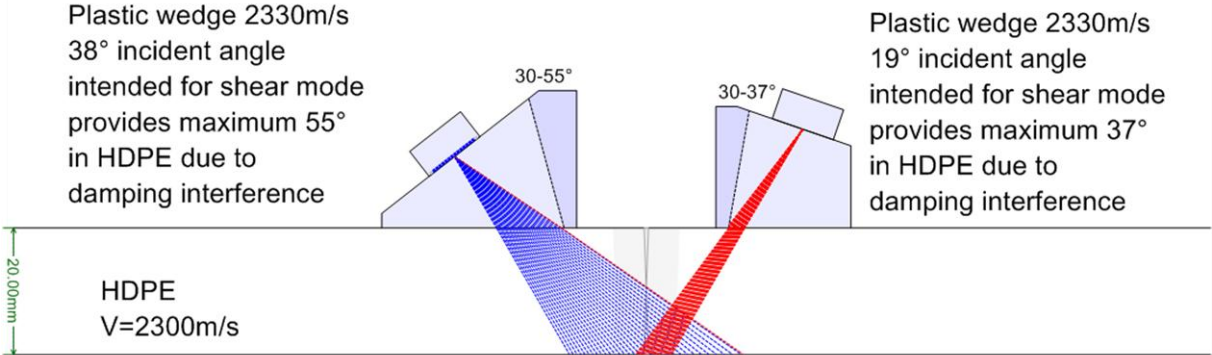
Figure 1 Limited sweep with hard-plastic refracting wedges on HDPE
